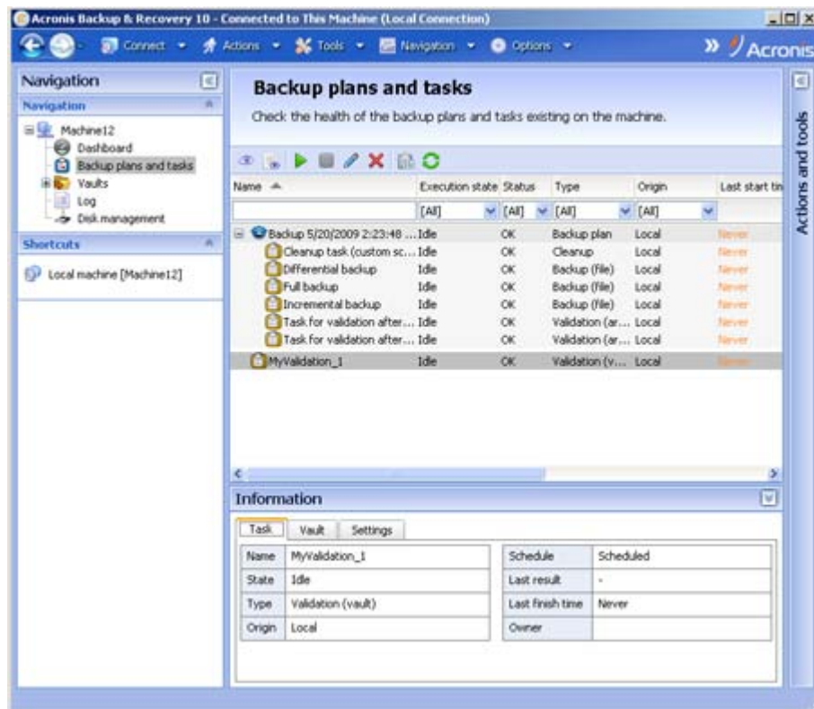
"Tasks" view
