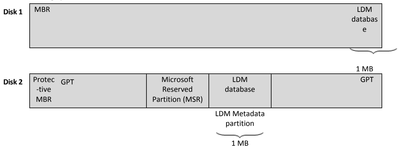
Dynamic disks organized on MBR (Disk 1) and GPT (Disk 2) disks.
